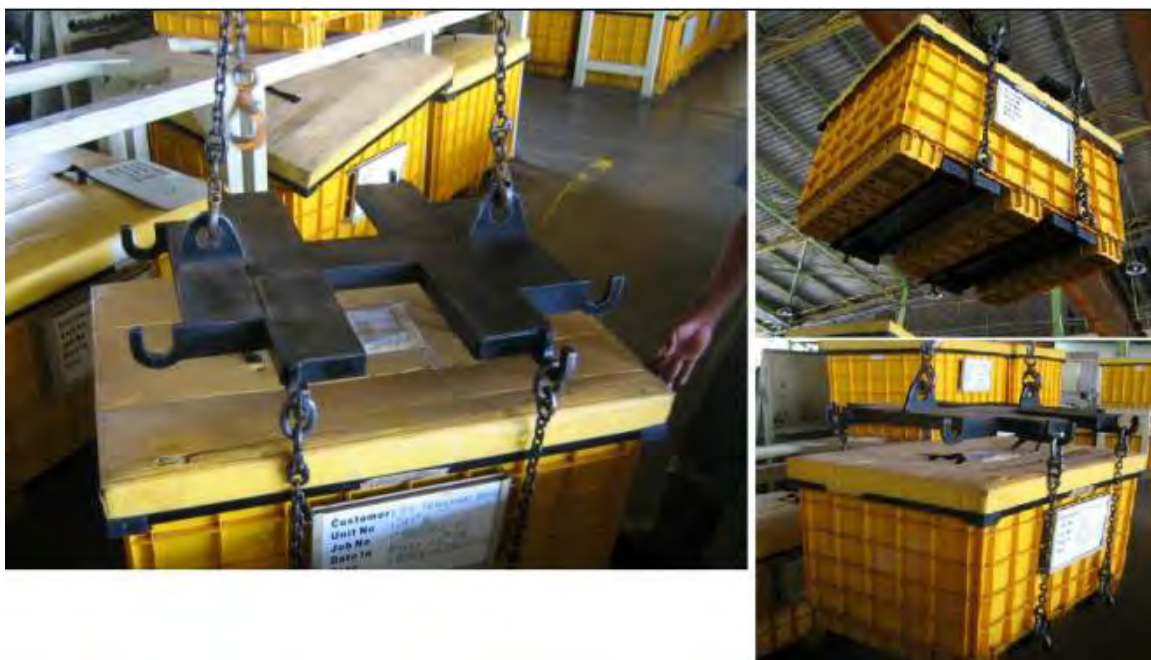
Figure 4, 5, and 6: Trakindo's WIP Parts Storage Box (yellow box) with fabricated lifting tool.
