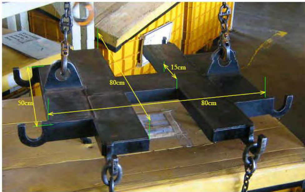
Figure 7: Top portion of lifting tool.
