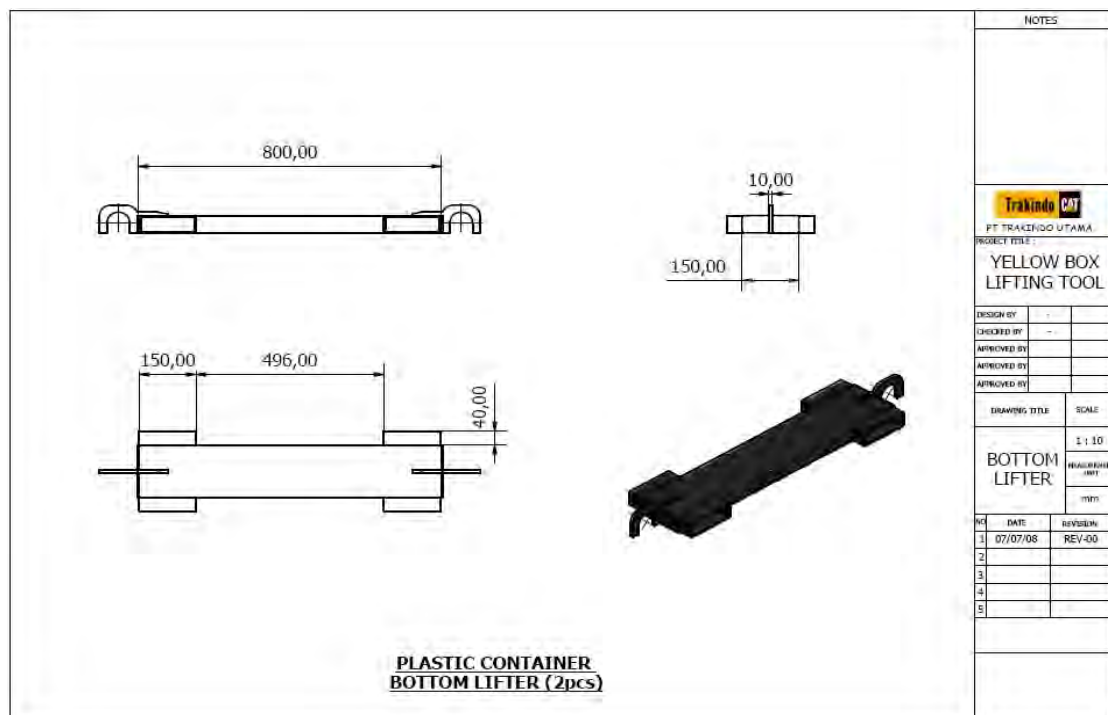
Figure 10: Drawing of bottom portion of lifting tool.
