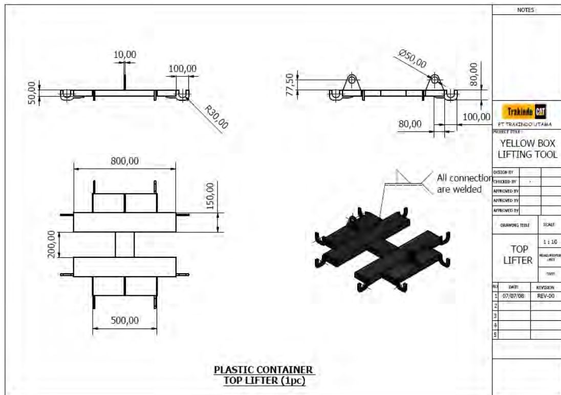
Figure 9: Drawing of top portion of lifting tool.
