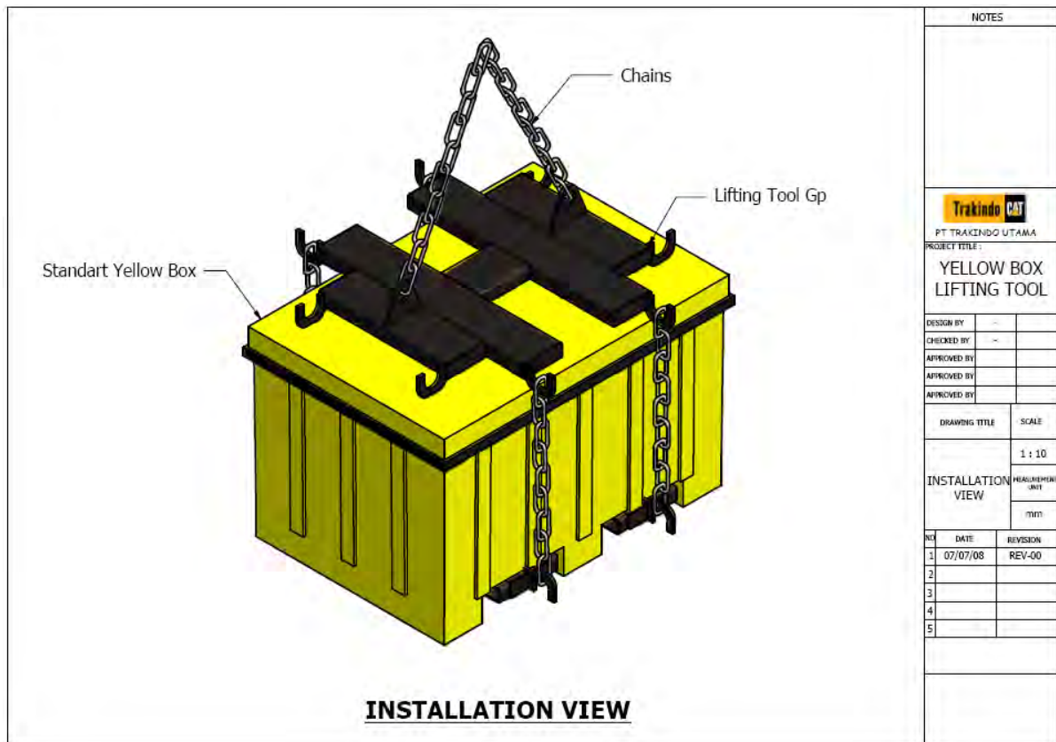
Figure 11: Drawing of lifting tool.
