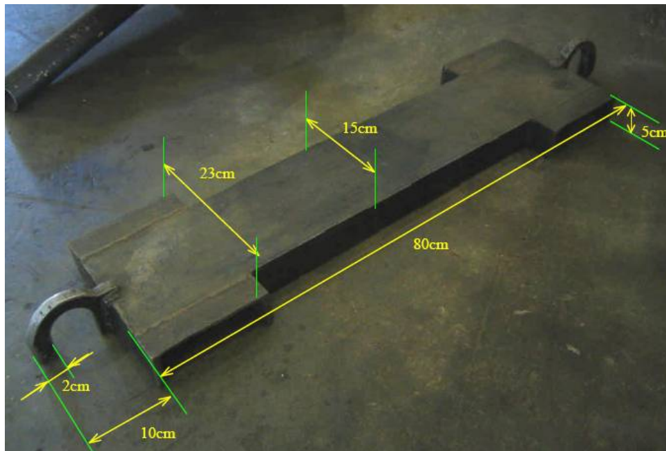
Figure 8: Bottom portion of lifting tool (2 pieces – see Figure 5).
